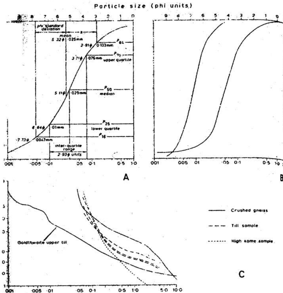
Figure : Cumulative frequency curves showing particle size distributions of sediments.
