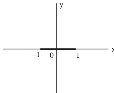
Fig. 50 Branch cut [-1, 1]
